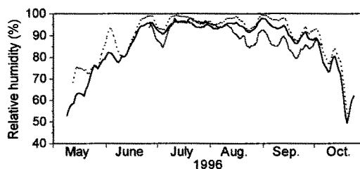
Fig. 3. The seven days running mean of relative humidity at BH (solid), LR (dotted) and YE (gray).
