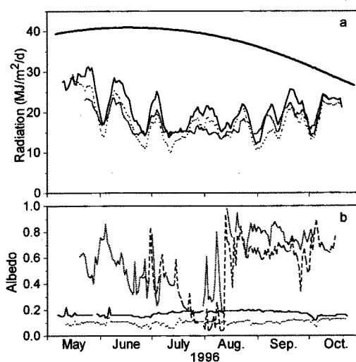
Fig. 6. a) The seven days running mean of daily mean short wave radiation at BH (solid), LR (dotted) and YE (gray) and at the top of atmosphere (thick solid). b) Daily mean albedo at BH (solid), LR (dotted), YE (gray) and YA (broken).
