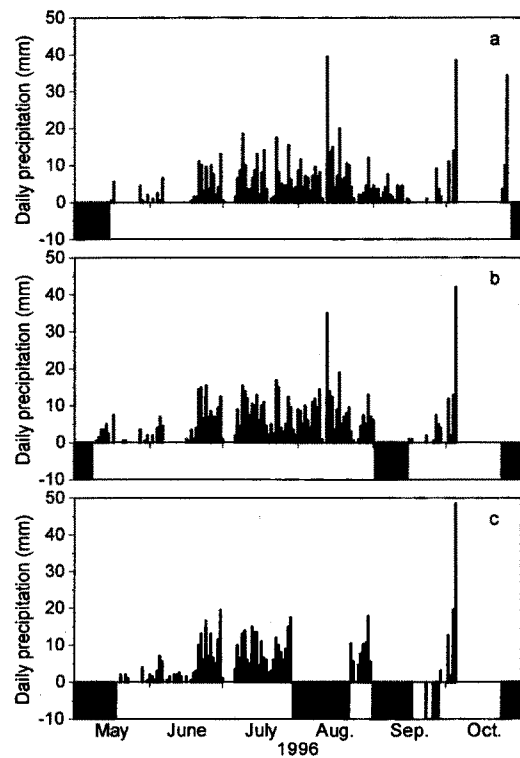
Fig. 5. Daily precipitation at YE (a), LR (b) and BH (c). The negative value denotes the data not available.
