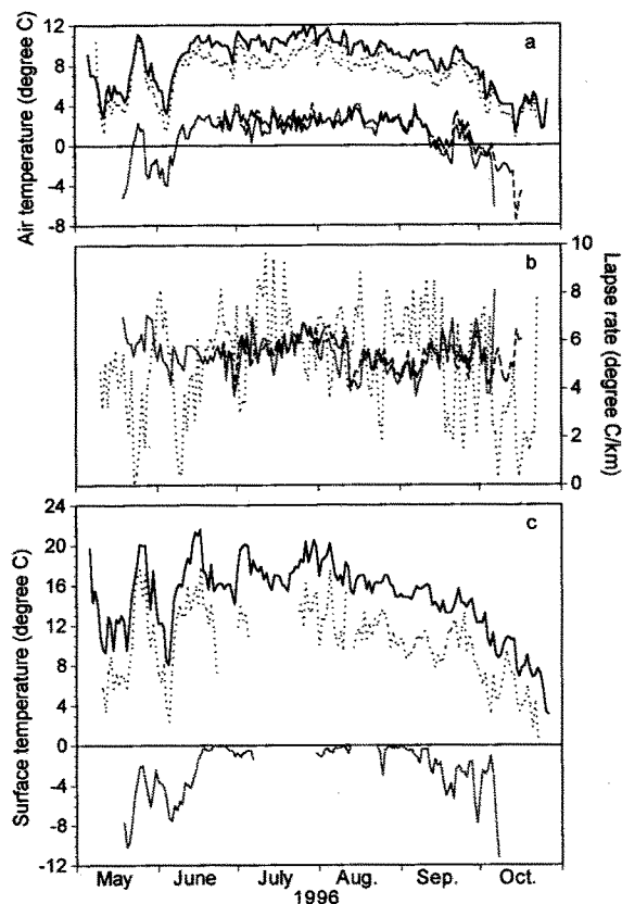
Fig. 2. a) Daily mean air temperature at BH, LR, YE and YA. b) Daily mean lapse rate with altitude at LR/BH, YE/BH and YA/BH. c) Daily mean surface temperature BH, LR and YE. The solid, dotted, gray and broken lines denote the parameters at BH, LR, YE and YA, respectively in all figures.
